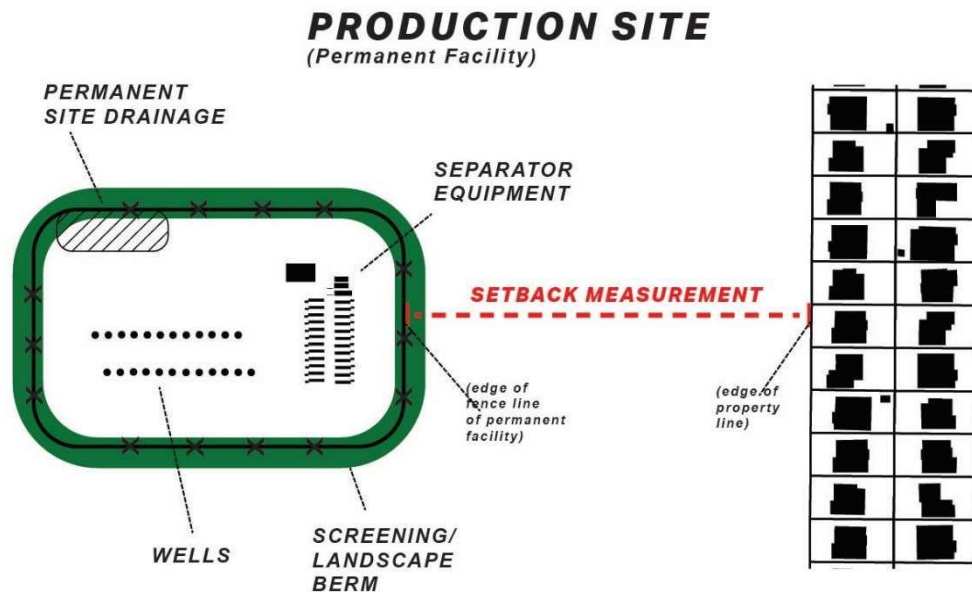
Figure V-4. Setback Measurement for Oil and Gas Facilities
