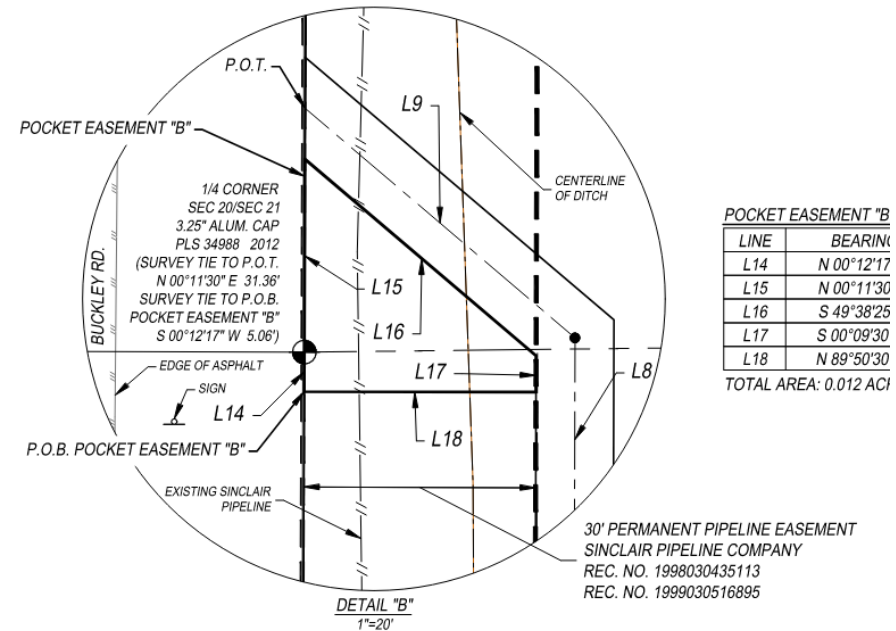
Detail B
