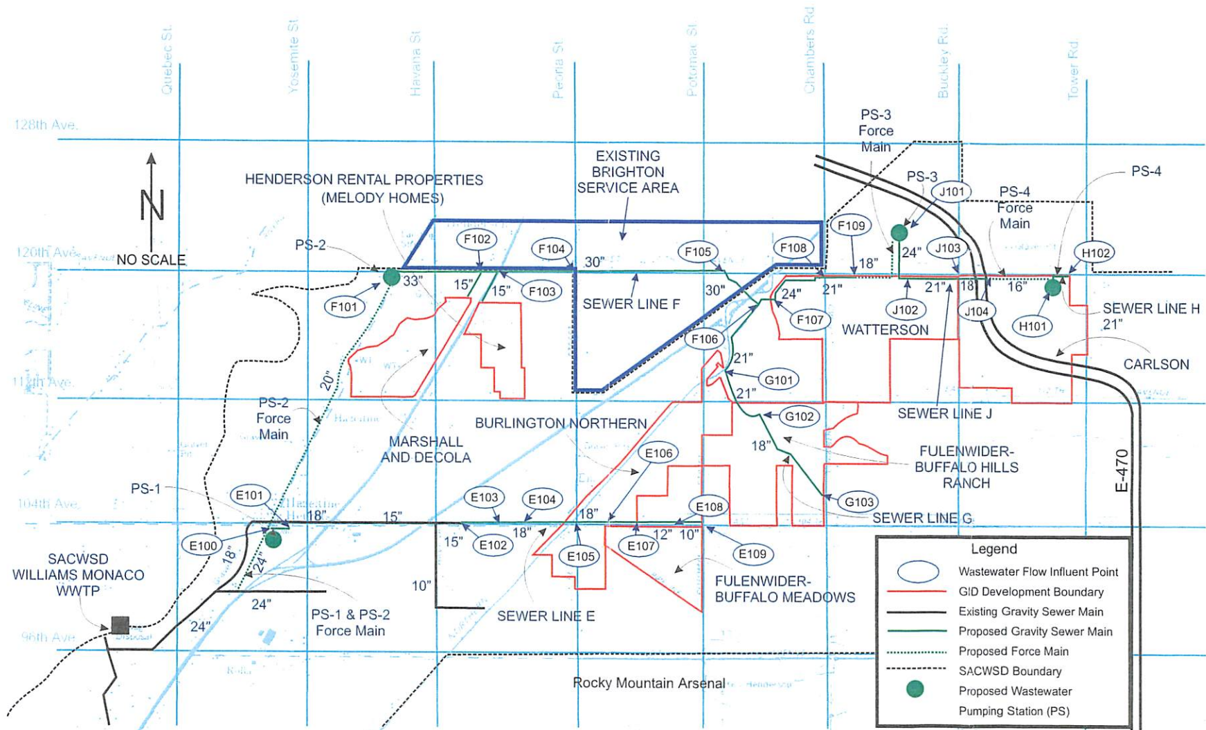
Figure 1 North Range Infrastructure Wastewater Collection System
