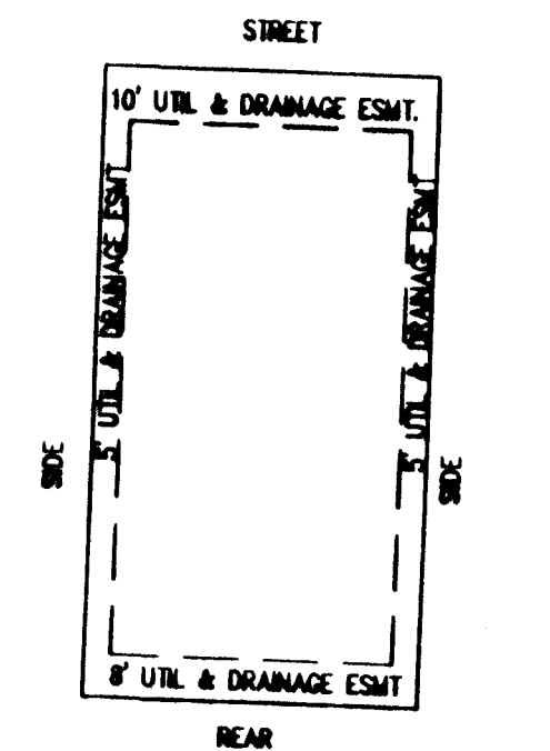
TYPICAL LOT EASEMENTS N.T.S.
