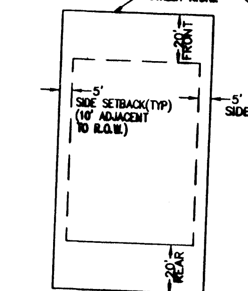
TYPICAL BUILDING SETBACK N.T.S.
