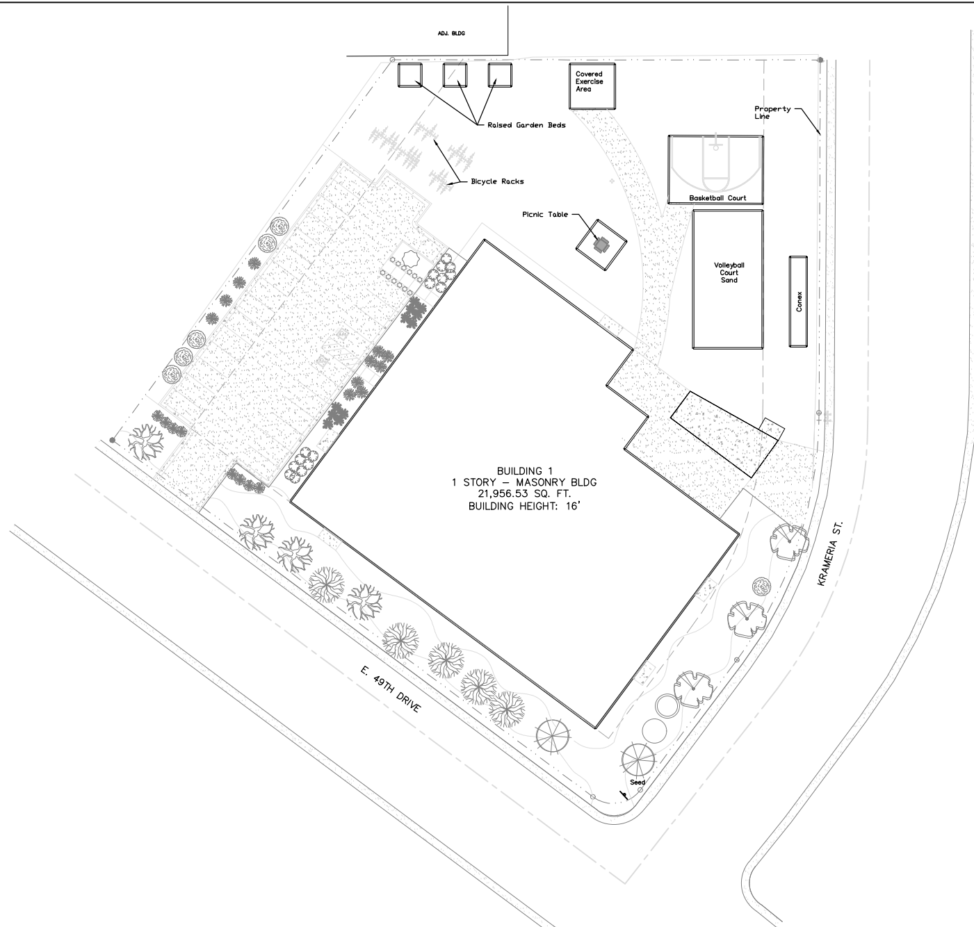
COMMERCE CITY TRANSITIONAL CENTER SITE PLAN
