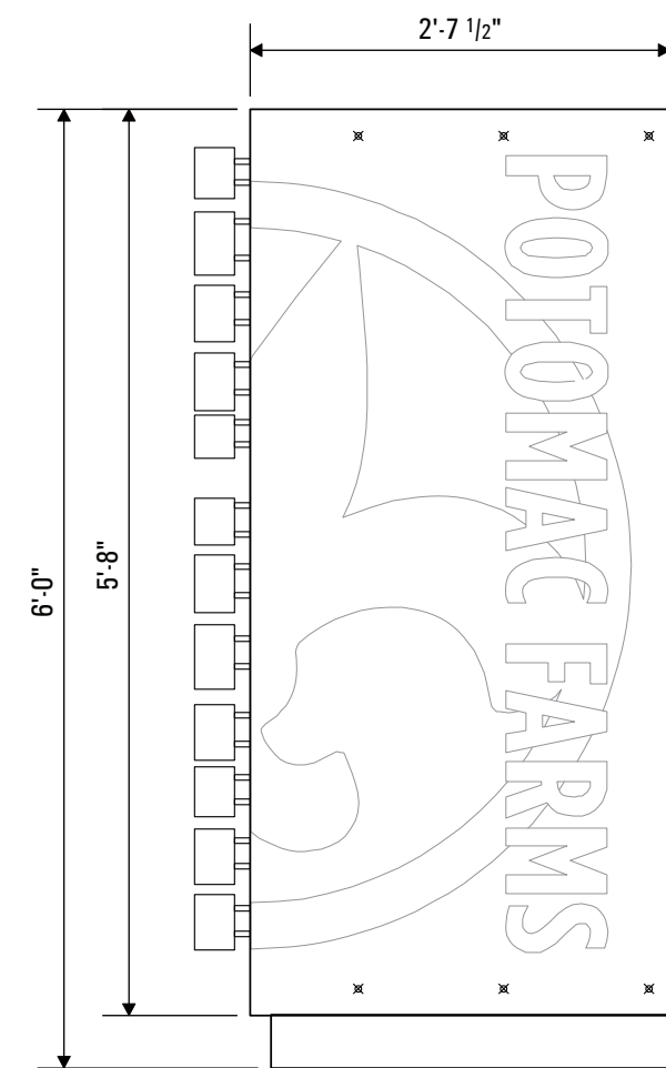
ELEVATION VIEW - PANEL SIGN SUBDIVISION ENTRYWAY IDENTIFICATION SCALE: 3/4" = 1'-0"
