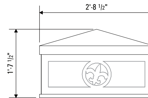
ELEVATION VIEW - LANTERN NON-SIGNAGE ELEMENT SCALE: 3/4" = 1'-0"
