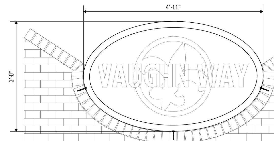
ELEVATION VIEW - LOGO METRO DISTRICT STREET SIGN SCALE: 3/4" = 1'-0"
