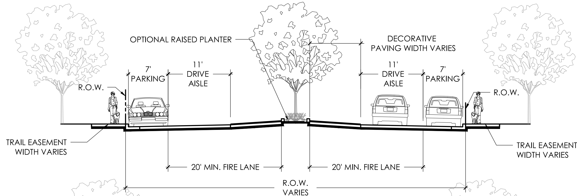
URBAN 2 LANE ROAD
