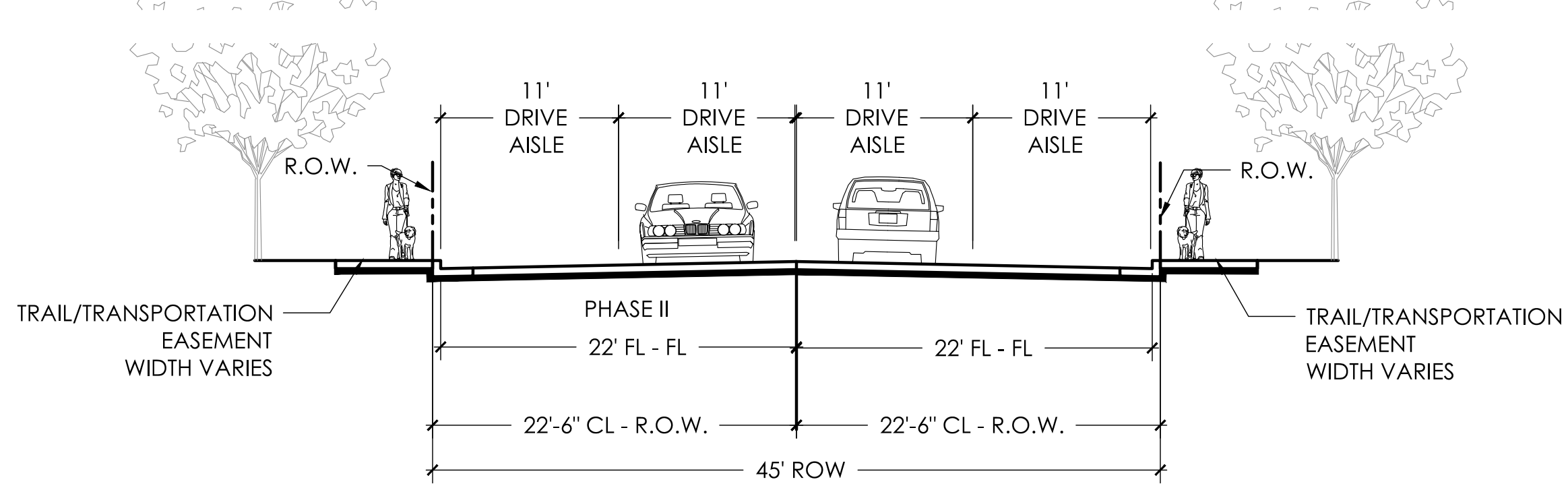
URBAN 4 LANE FINAL CONDITION
