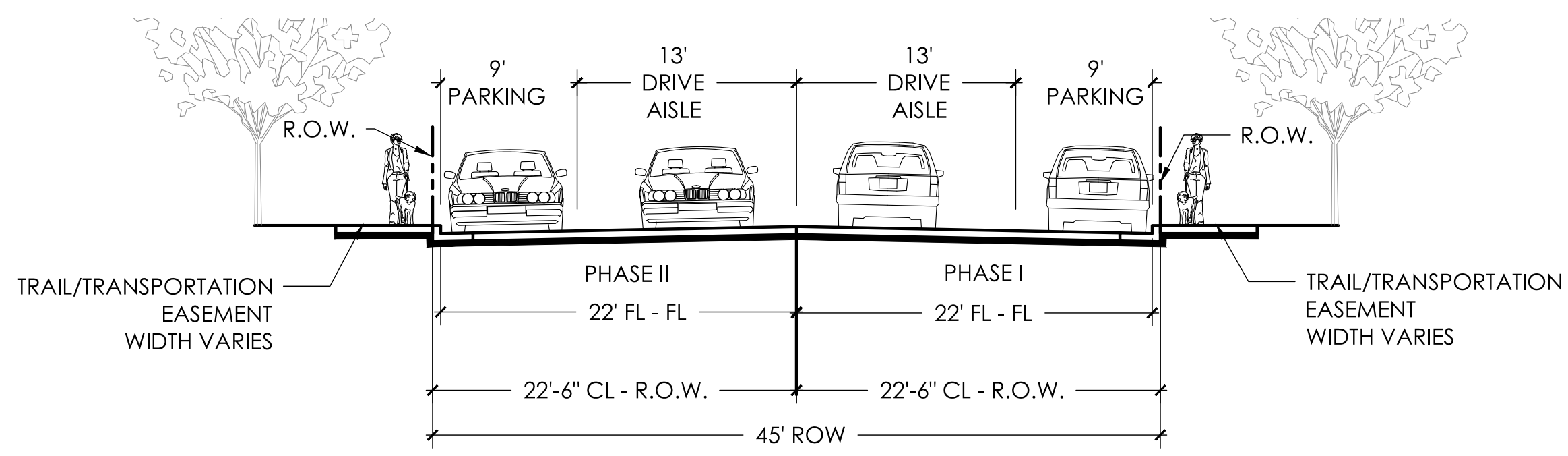
URBAN 4 LANE INTERIM CONDITION
